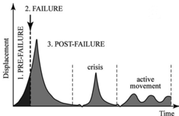
Figure 5: Classification of landslides according to their movement phase [van Asch et al. , 2007], modified after [Vaunat et al. , 1994].
